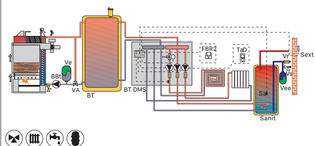
KIT BT 2M + BT
