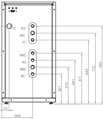
FUSION COMBI F 80
