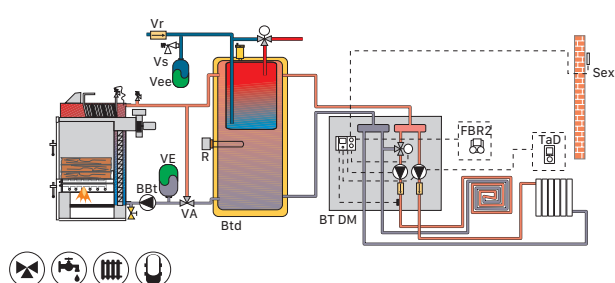
KIT BT DM + BT DUO
