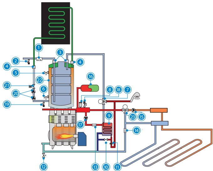
SIRENA SOLAR HFD + KIT SRS2
