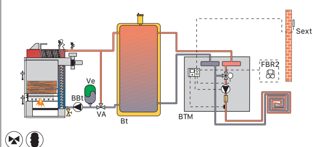
KIT BT DMS + BT
