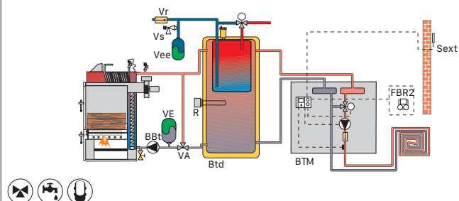
KIT BT 2M + BT DUO
