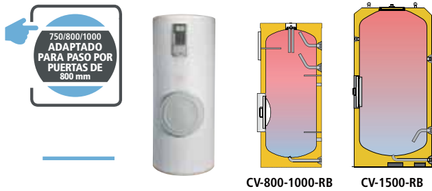
CV-800-1000-RB
